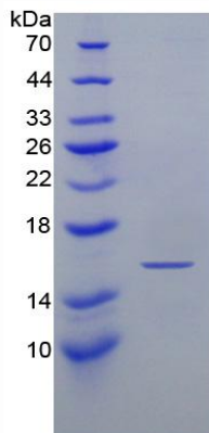
Figure 2. SDS-PAGE
